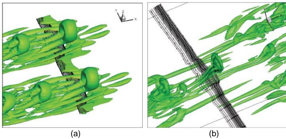
Figure 3-4 Comparison of our DNS results with Rist's DNS data using \lambda_2 and vortex filaments (a) Our DNS (b) Rist's DNS
