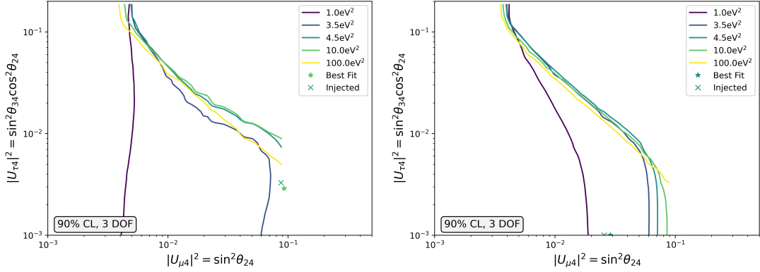
FIGURE 7.5.8: Two signal inject-recover tests.
