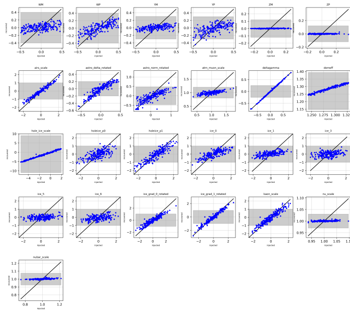
FIGURE 7.5.2: Fit results after injecting various perturbed values for each nuisance parameter and running the fitter. A shaded gray region demonstrates the 1\sigma prior width on the nuisance parameter's prior.
